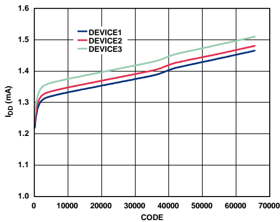
Figure 35. I_{DD} vs. Code
