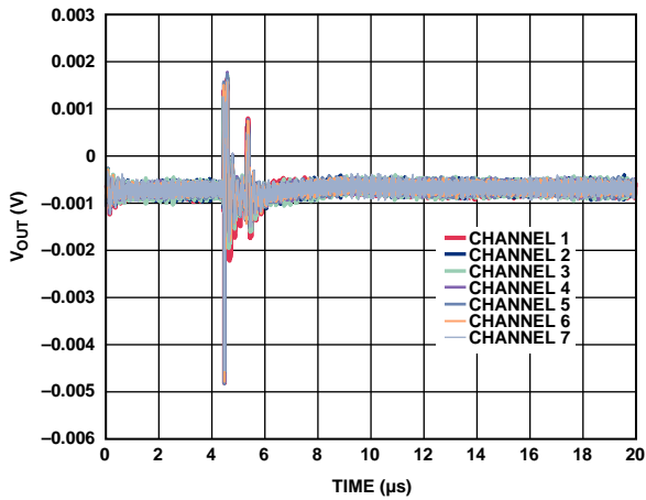
Figure 43. Analog Crosstalk
