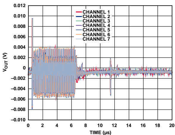
Figure 44. DAC-to-DAC Crosstalk
