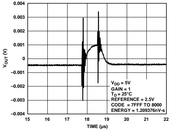
Figure 42. Digital-to-Analog Glitch Impulse
