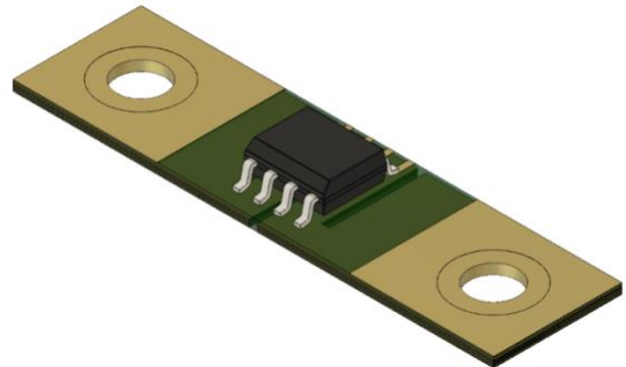
Figure 18. 3D View of CT452 and PCB Trace Design
