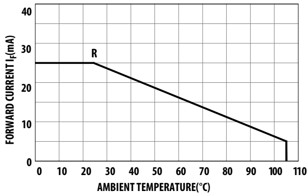
Figure 11: Allowable DC Current vs. Ambient Temperature
