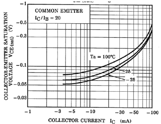
Fig. 10.20 RN2302 V_{CE(sat)}-I_C
