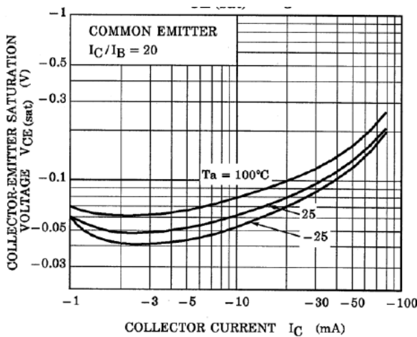
Fig. 10.21 RN2303 V_{CE(sat)}-I_C
