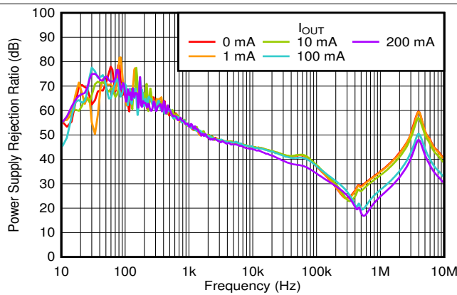
Figure 44. PSRR vs Frequency and I_{OUT}
