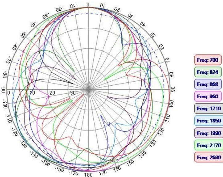
XZ - Plane
