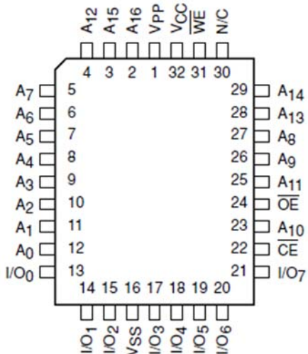
PLCC Package
