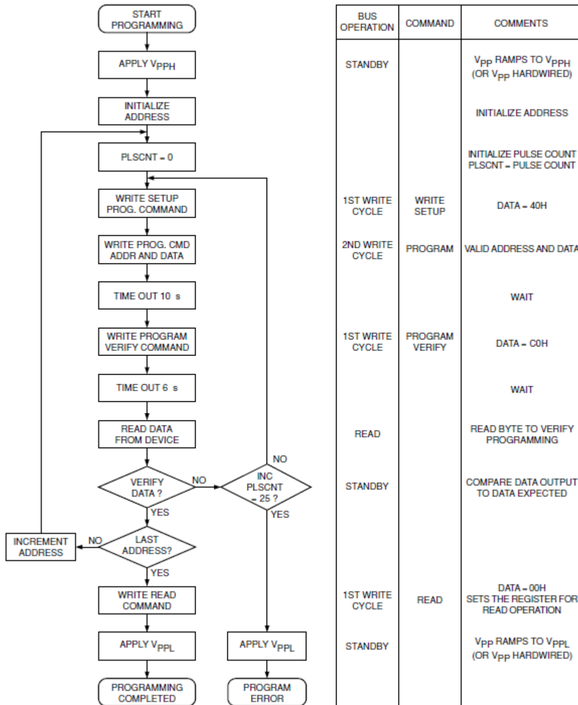
Figure 7. Programming Algorithm (1)
