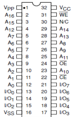
PDIP Package
