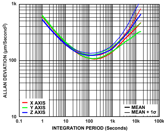
Figure 15. Accelerometer Allan Deviation, T_c = 25^\circ\text{C}
