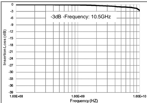
Fig.5 Insertion Loss
