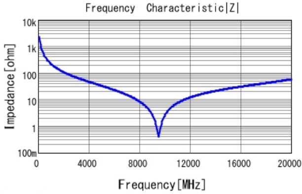
GJM1555C1HR70BB01 |Z| DCOV, 25degC
