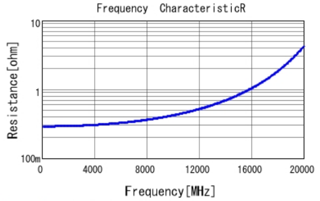
GJM1555C1HR70BB01 R DCOV, 25degC
