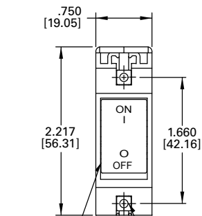
OPTIONAL GUARD (SEE DETAIL "A") 6-32 THD. MOUNTING M3 ISO THD. OPTIONAL
