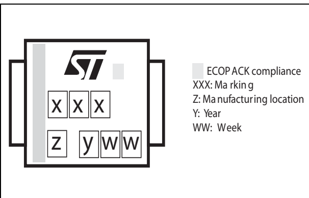
Figure 12. Marking layout (1)
