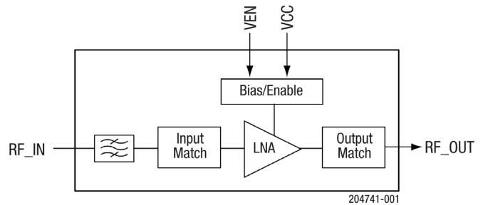
Figure 1. SKY65728-11 Block Diagram
