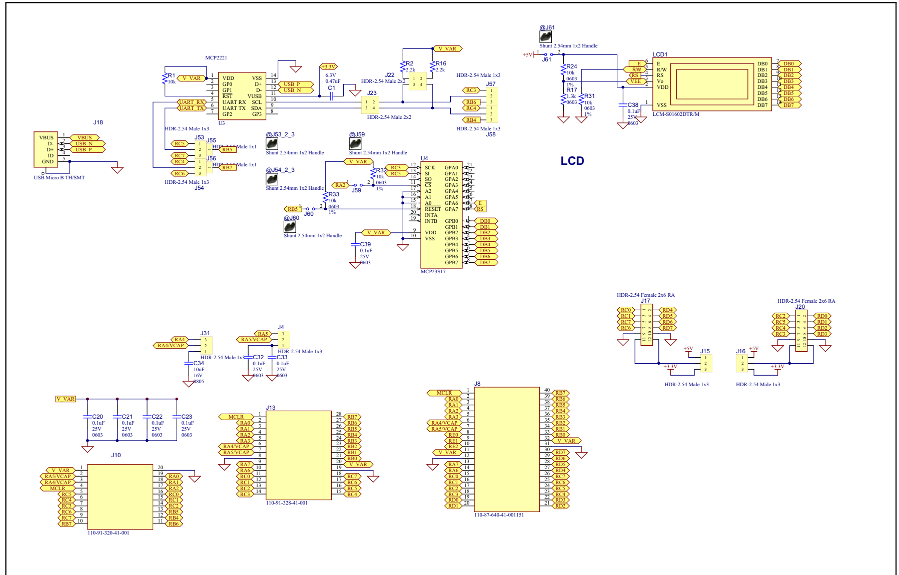
FIGURE A-4: EXPLORER 8 DEVELOPMENT SCHEMATIC - 3
