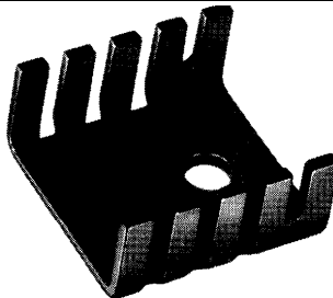
FK 239 / SA-32 24 K/W
