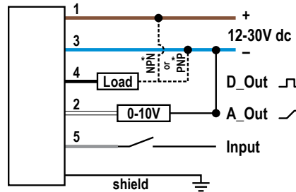
Figure 5. Analog Voltage Model
