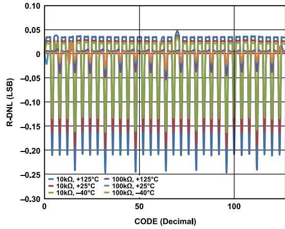
Figure 10. R-DNL vs. Code (AD5122A)
