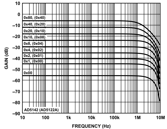
Figure 22. 100 \text{k}\Omega Gain vs. Frequency and Code
