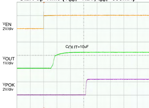
Start-up Time ( V_{OUT}=1.2V , I_{OUT}=600mA )
