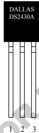
TO-92
