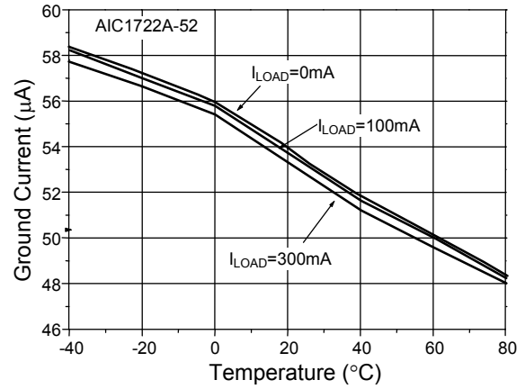
Fig. 8 Ground Current vs. Temperature
