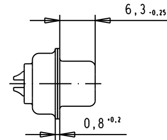
Solder buckets for AWG 20 Max
