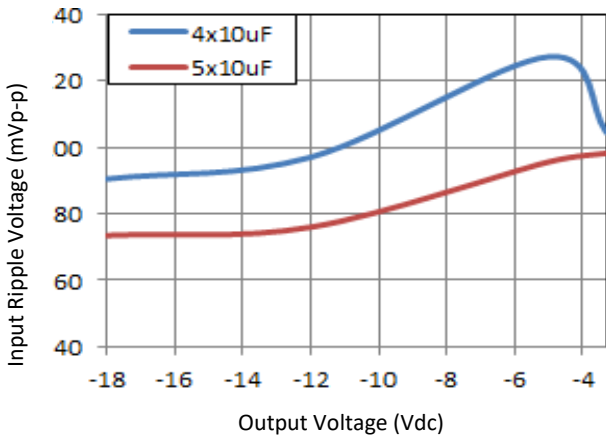
Figure 64. Input ripple voltage with 4x10 \mu F or 5x10 \mu F ceramic capacitors at the input (max load).
