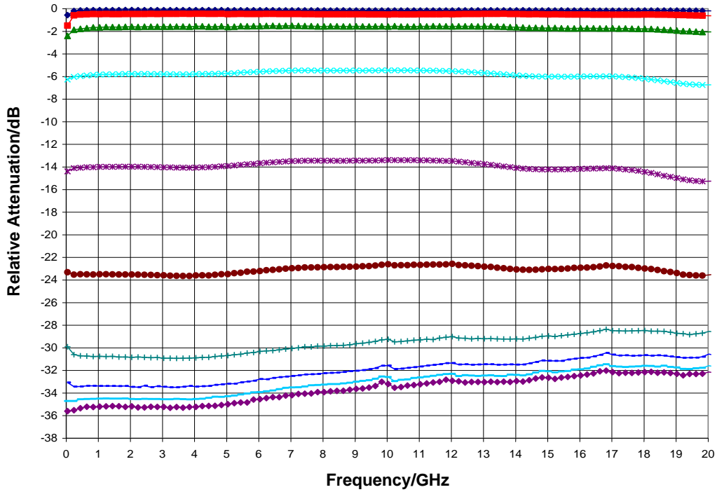
Relative Attenuation, Complementary Control Voltage Table, T_A = 25^\circ C
