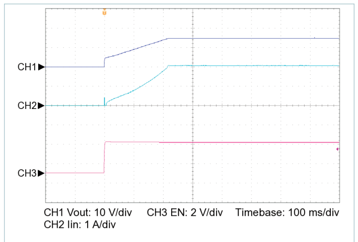
Figure 14 — Startup from EN, V_{IN} = 42\text{ V} , C_{OUT\_EXT} = 10000\ \mu\text{F} , R_{LOAD} = 2.778\ \Omega
