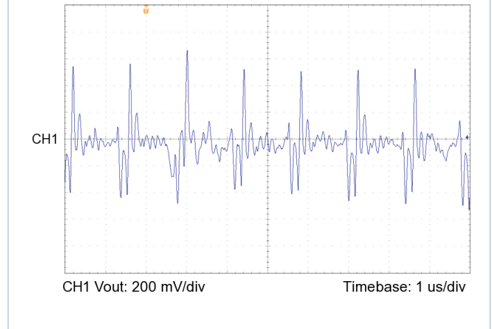
Figure 16 — Output voltage ripple, V_{IN} = 42\text{ V} , V_{OUT} = 15.0\text{ V} , C_{OUT\_EXT} = 1000\ \mu\text{F} , R_{LOAD} = 2.778\ \Omega
