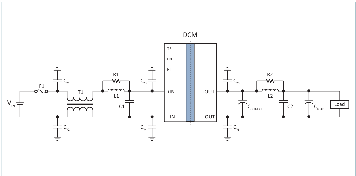
Typical Application 2: Single DCM3623x75X1780y7z with common- and differential-mode input filters
