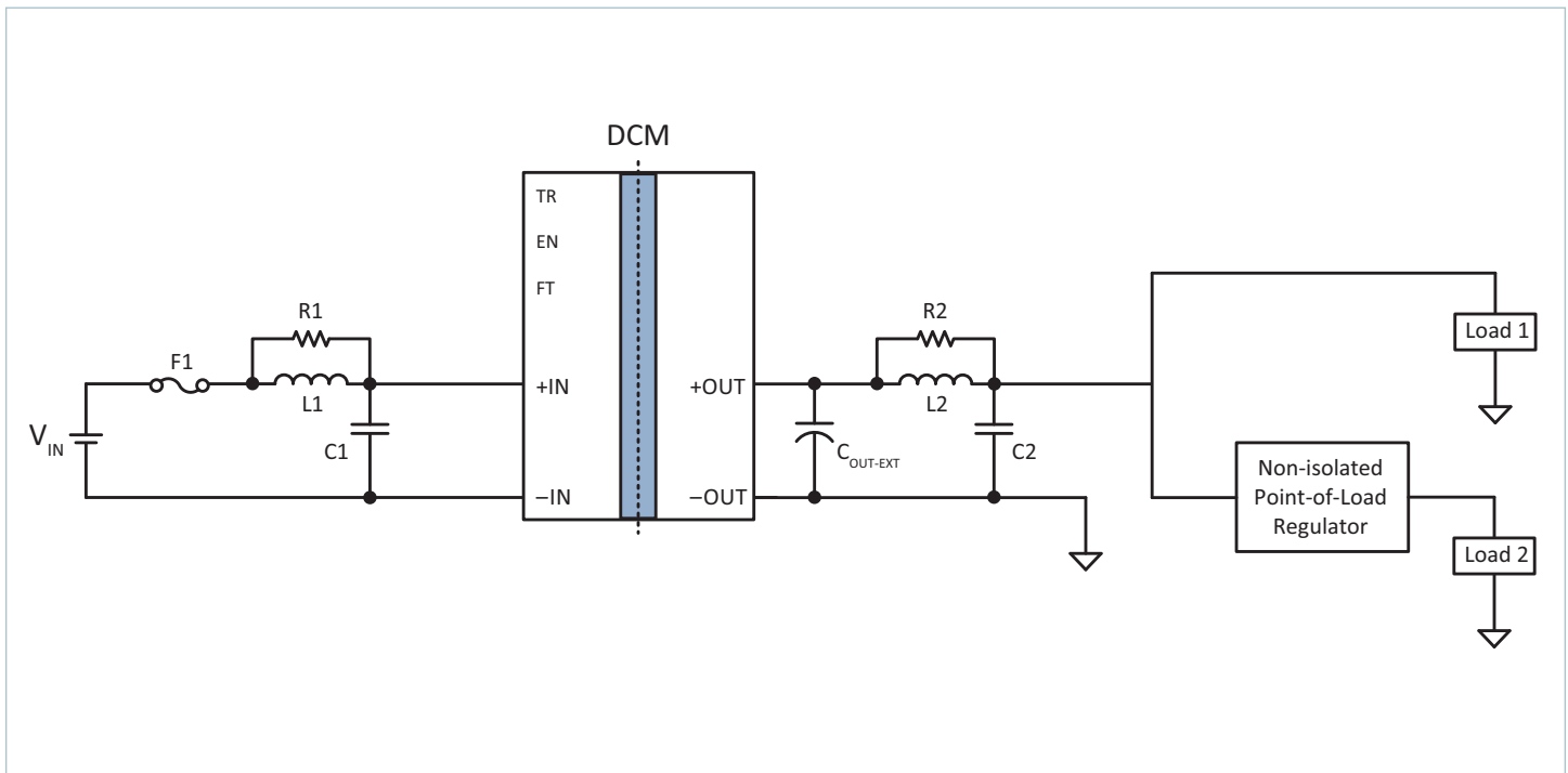
Typical Application 1: Single DCM3623x75X1780y7z, to a non-isolated regulator, and direct to load
