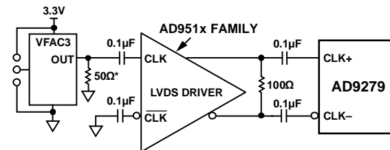
Figure 55. Differential LVDS Sample Clock
