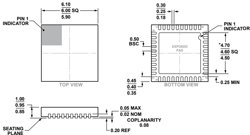
*COMPLIANT TO JEDEC STANDARDS MO-220-VJJD-5 WITH THE EXCEPTION OF THE EXPOSED PAD DIMENSION. Figure 94. 40-Lead Lead Frame Chip Scale Package [LFCSP] 6 mm × 6 mm Body and 0.95 mm Package Height (CP-40-15) Dimensions shown in millimeters
