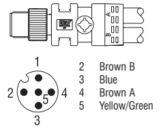
WIRING CONFIGURATION
