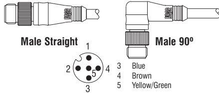
WIRING CONFIGURATION
