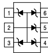
PIN 1. CATHODE 2. ANODE 3. CATHODE 4. CATHODE 5. CATHODE 6. CATHODE
