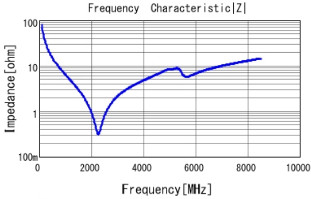
GRM0335C1E200JA01 |Z| DCOV, 25degC
