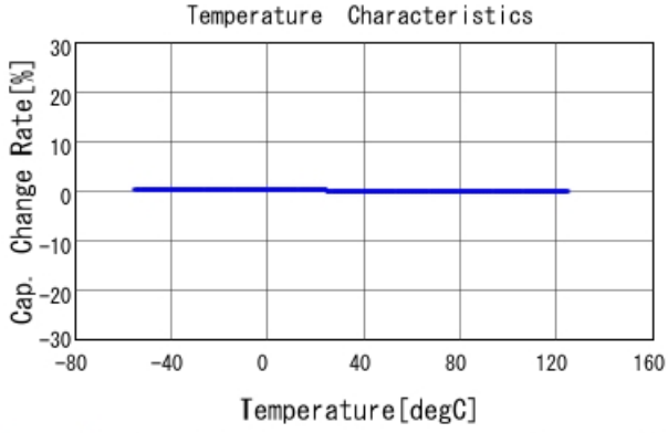
GRM0335C1E200JA01 C-Temp. capchange, DCOV, AC1Vrms
