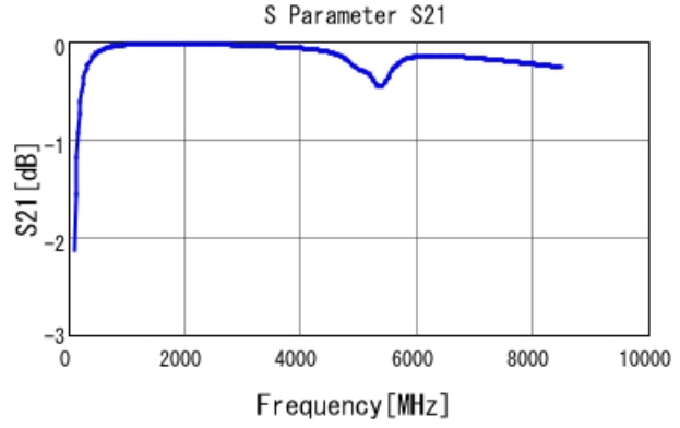
GRM0335C1E200JA01 S21 DCOV, 25degC
