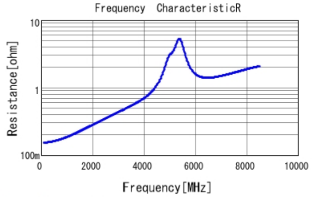
GRM0335C1E200JA01 R DCOV, 25degC
