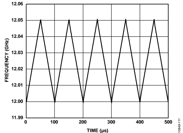
Figure 11. Triangle Ramp, f_{PD} = 100 MHz, I_{CP} = 2.5 mA, Loop Bandwidth = 250 kHz, CLK_1 = 3 , CLK_2 = 26 , DEV = 1024 , DEV\_OFFSET = 8 , Number of Steps = 64
