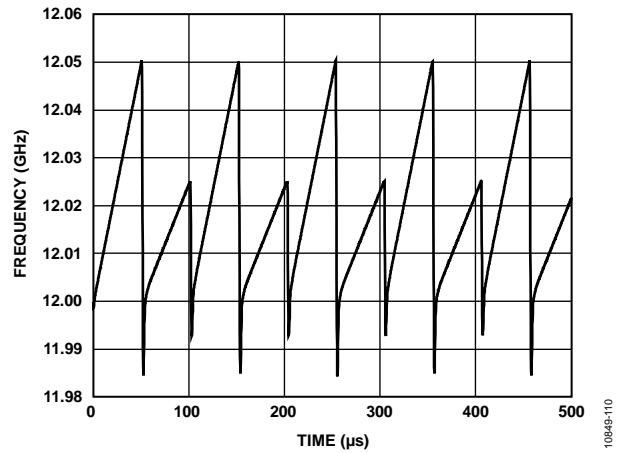
Figure 10. Dual Sawtooth Ramp, f_{PD} = 100 MHz, I_{CP} = 2.5 mA, Loop Bandwidth = 250 kHz, CLK_1 = 3 ; First Ramp: CLK_2 = 26 , DEV = 1024 , DEV\_OFFSET = 8 , Number of Steps = 64; Second Ramp: CLK_2 = 52 , DEV = 1024 , DEV\_OFFSET = 7 , Number of Steps = 64
