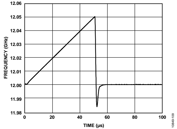
Figure 9. Sawtooth Burst, f_{PD} = 100 MHz, I_{CP} = 2.5 mA, Loop Bandwidth = 250 kHz, CLK_1 = 3 , CLK_2 = 26 , DEV = 1024 , DEV\_OFFSET = 8 , Number of Steps = 64
