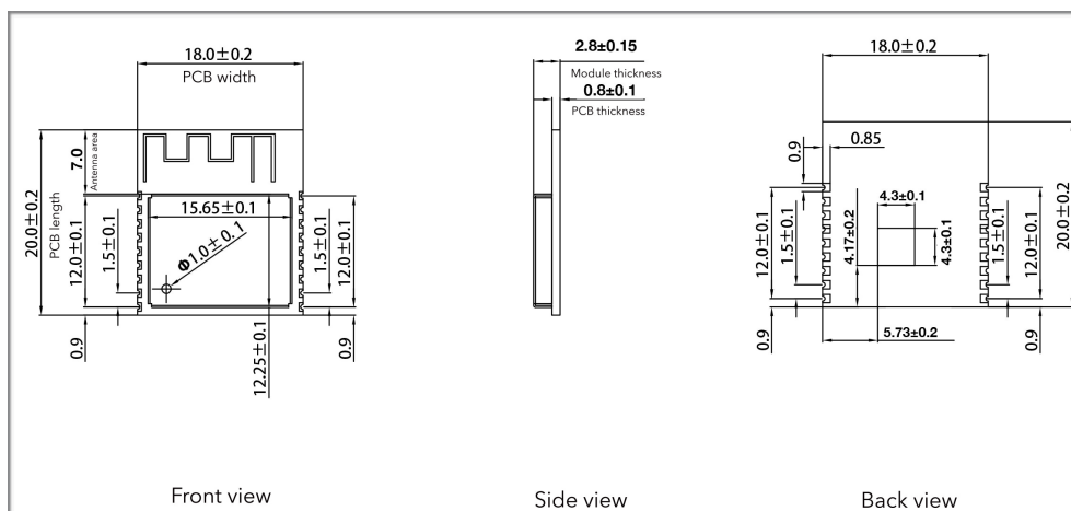
Figure 6-1. Dimensions of ESP-WROOM-02
