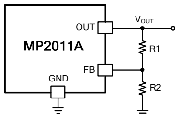
Figure 2: FB Resistor Divider to Set V_{OUT}
