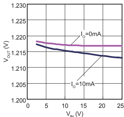
V_{OUT} vs. V_{IN} V_O = 1.215V
