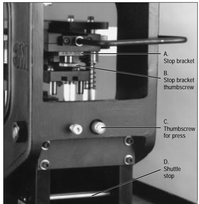
Figure 2. Back of press
