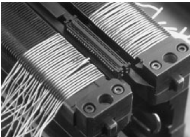
Figure 10. Cut wires
