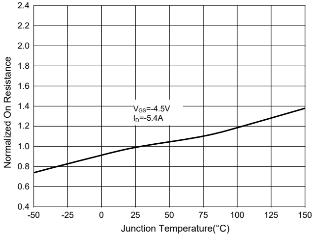
Fig.7-NormalizedOnResistanceCharacteristics
