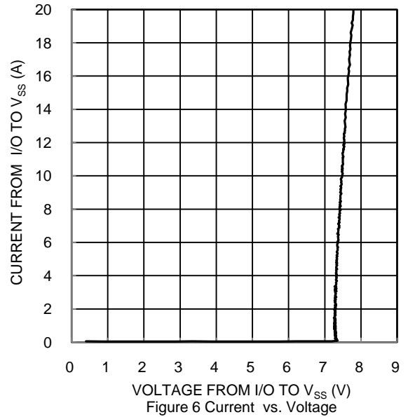
Figure 6 Current vs. Voltage
