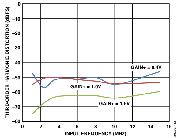
Figure 15. Third-Order Harmonic Distortion vs. Frequency, AOUT = -1.0 dBFS
