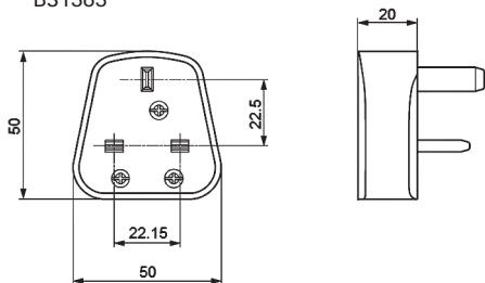
BS1363
