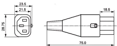
C13
