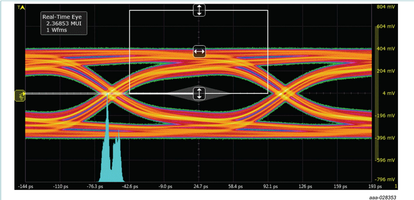
Figure 9. HDMI 2.0 eye diagram TP1, test board with PCMFxUSB3B/C; typical values
