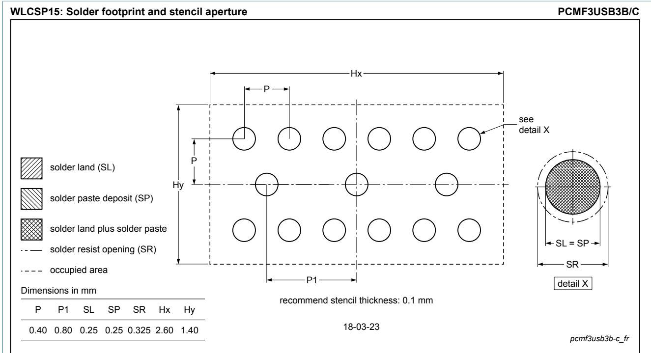
Figure 25. Soldering footprint WLCSP15 (PCMF3USB3B/C)
