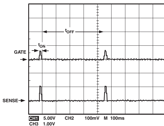
Figure 11. Illustration of the PWM Ratio ( t_{ON}/t_{OFF} )
