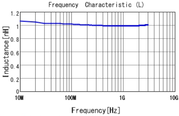
LQG15HN1N0S02 L
