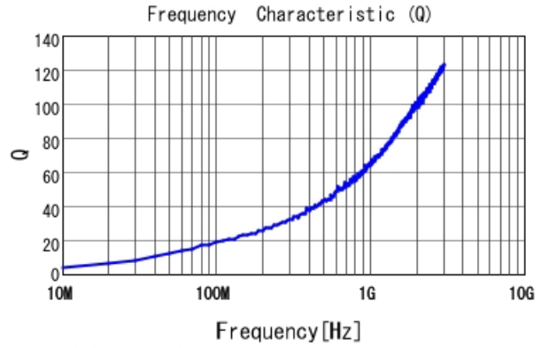
LQG15HN1N0S02 Q
