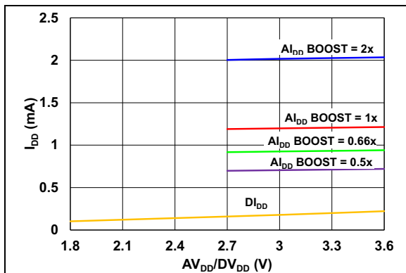
FIGURE 2-55: D I_{DD} and A I_{DD} vs. DV_{DD} and AV_{DD} .
