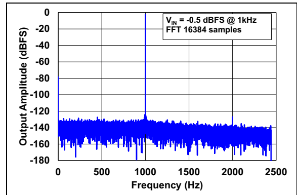
FIGURE 2-4: FFT Output Spectrum, f_{in} = 1 kHz (Internal V_{REF} ).
