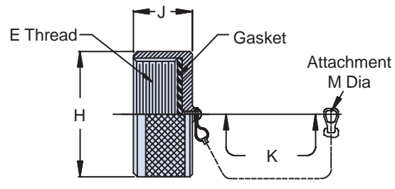
MS25043 Receptacle Cover
