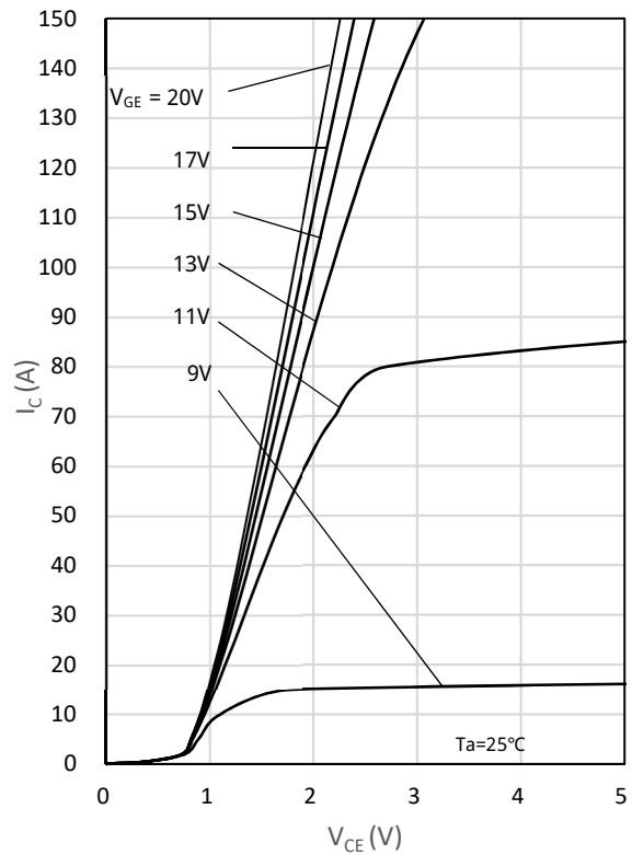
Fig. 2 Output characteristics
