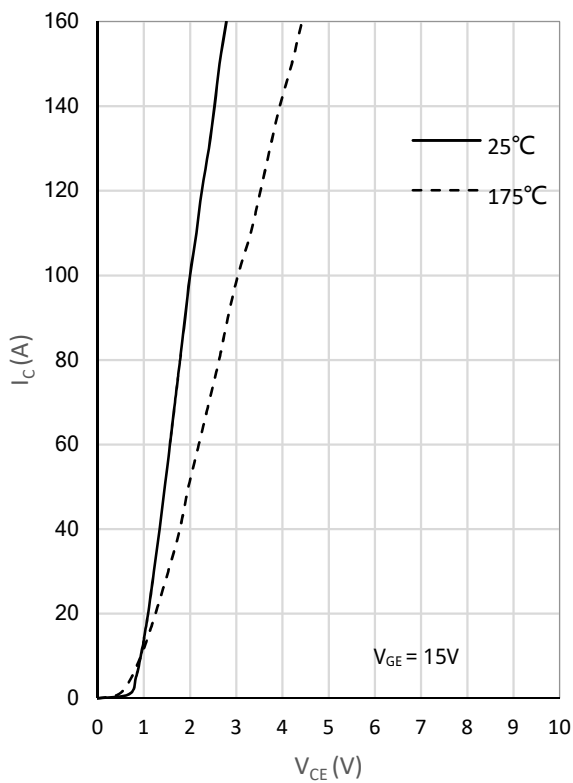
Fig. 3 Saturation voltage characteristics
