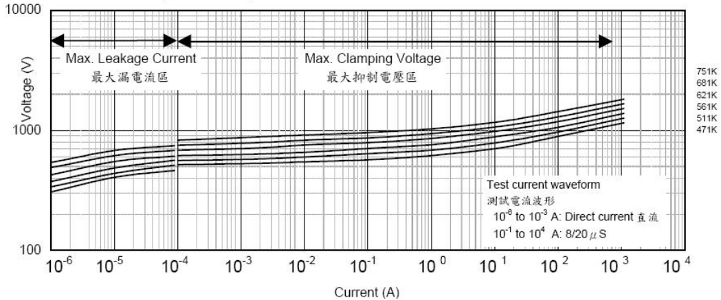
VDR-10D471K-10D112K(N/J SERIES)
