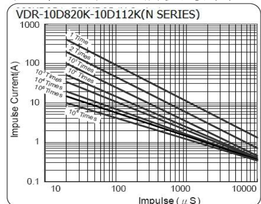
Surge Life Time Ratings 額定突波壽命 N (Standard)/K (Low Capacitance) Series 標準型/低電容系列
