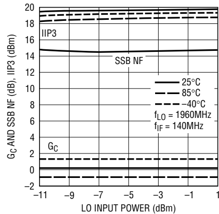
Conv Gain, IIP3 and SSB NF vs LO Power (RF = 2100MHz)
