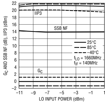
Conv Gain, IIP3 and SSB NF vs LO Power (RF = 1800MHz)
