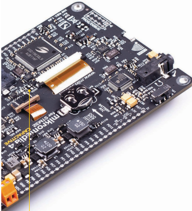
Figure 16: mikromedia 4 partial back view
