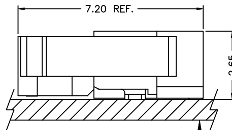
MATED CONDITION
