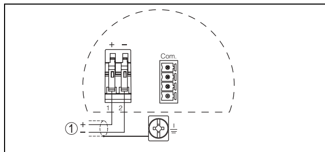
Fig. 6: Connection HART, Profibus PA, Foundation Fieldbus two-wire
