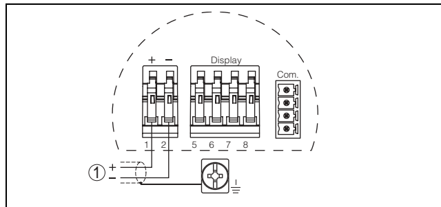
Fig. 5: Connection HART two-wire, Profibus PA, Foundation Fieldbus
