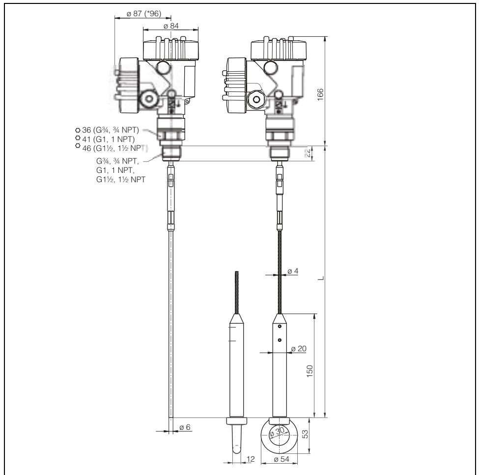
Fig. 16: VEGAFLEX 61 - Cable and rod version with thread (double chamber housing)
