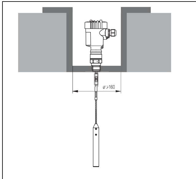
Fig. 4: Installation in concrete silos
