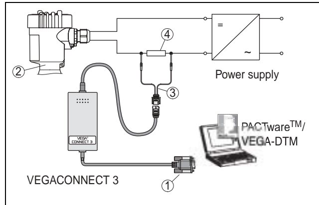
Fig. 10: Connecting the PC to the signal cable
