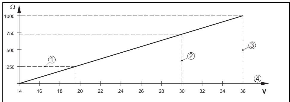
Fig. 13: Voltage diagram
