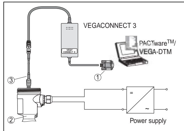
Fig. 9: PC connected directly to the sensor
