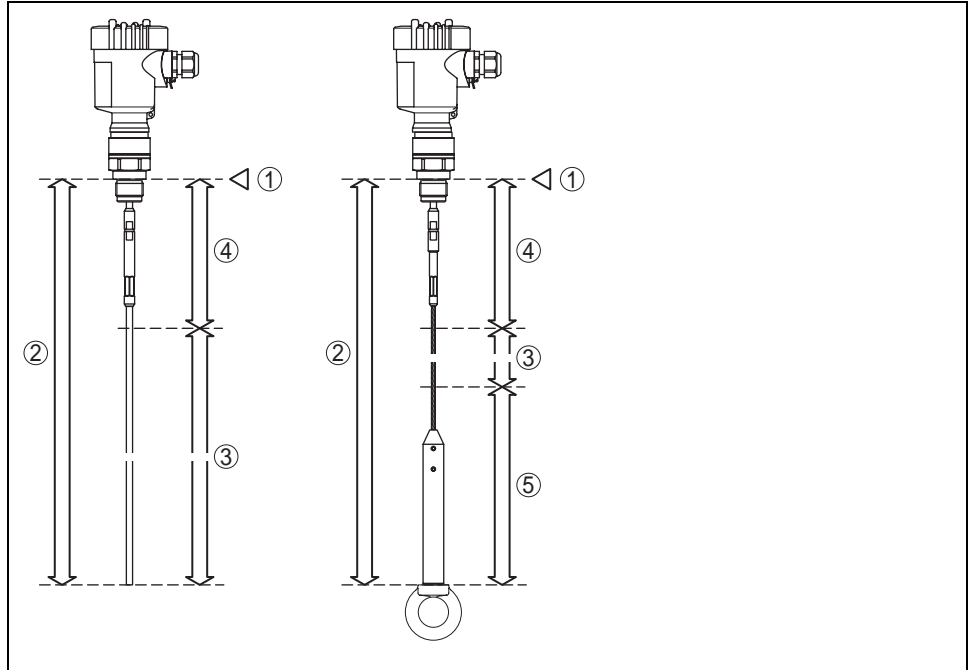
Fig. 11: Meas. ranges of VEGAFLEX - rod and cable version e.g. VEGAFLEX 61
