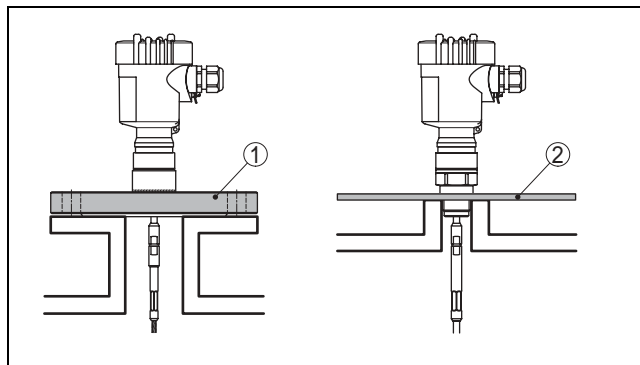
Fig. 3: Installation in plastic silo
