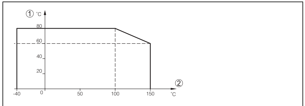
Fig. 12: VEGAFLEX - Ambient temperature - Product temperature
