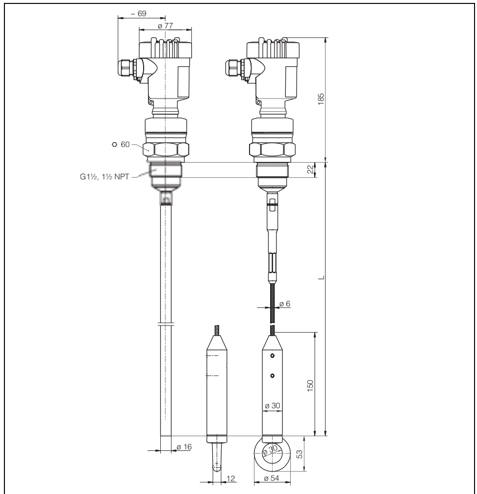
Fig. 17: VEGAFLEX 62 - Cable and rod version with thread
