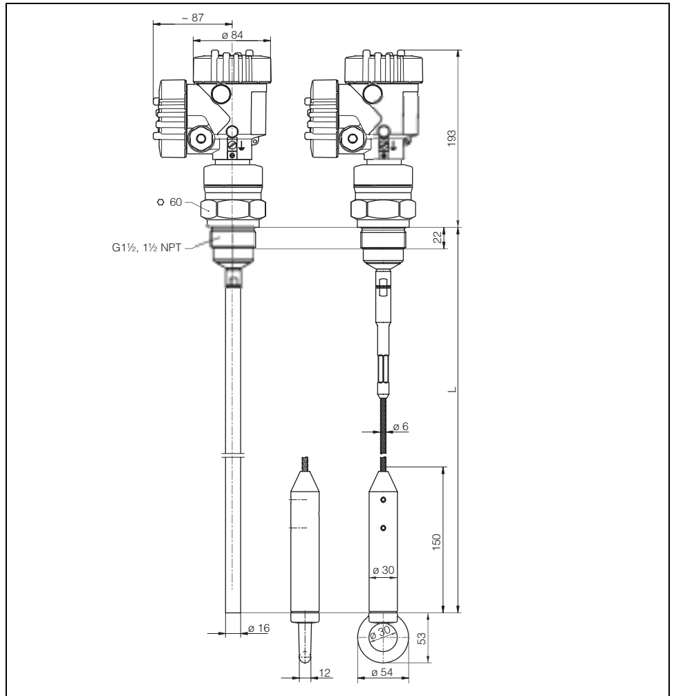
Fig. 18: VEGAFLEX 62 - Cable and rod version with thread (double chamber housing)
