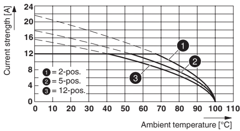
Type: FKCN 2,5/...-ST-5,08 with MSTBVA 2,5/...-G-5,08
