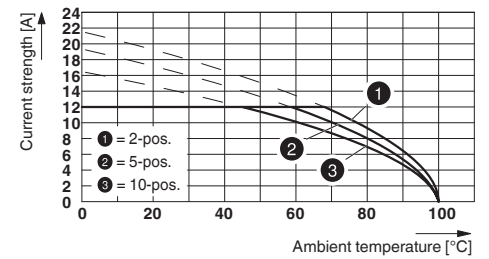
Type: TFKC 2,5/...-ST-5,08 with MSTBVA 2,5/...-G-5,08
