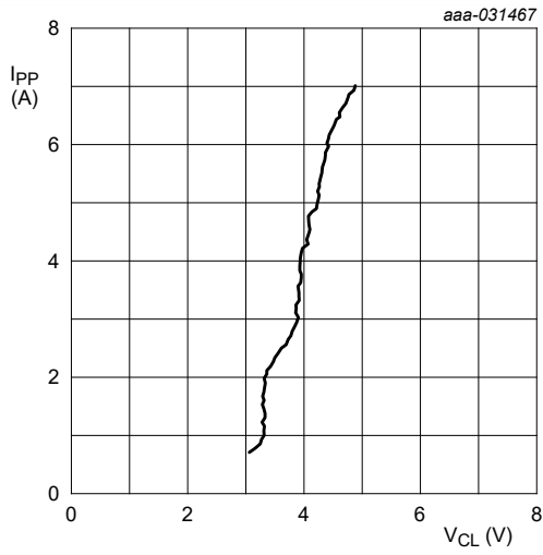
Fig. 16. Dynamic resistance with positive clamping; typical values
